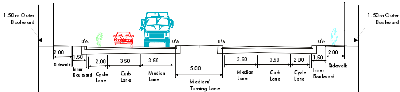
Typical 4-lane Cross Section Orléans Boulevard to Trim Road (34 metre Right-of-way*)
