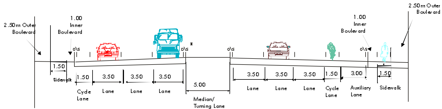
Typical 6-lane Cross Section Highway 417 to Blair (43 metre Right-of-way*)
