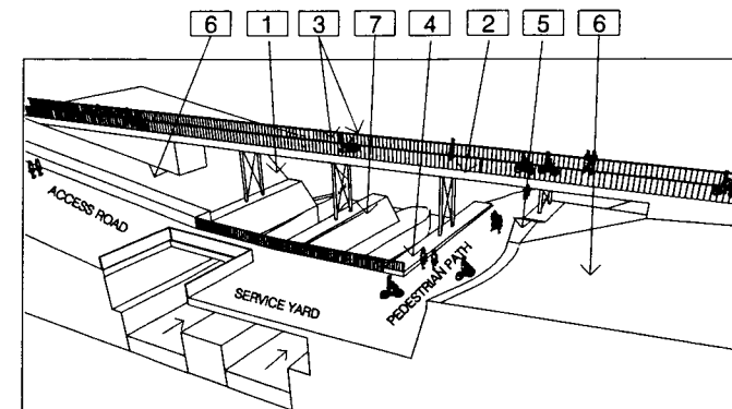
PERSPECTIVE VIEW FROM SOUTH
