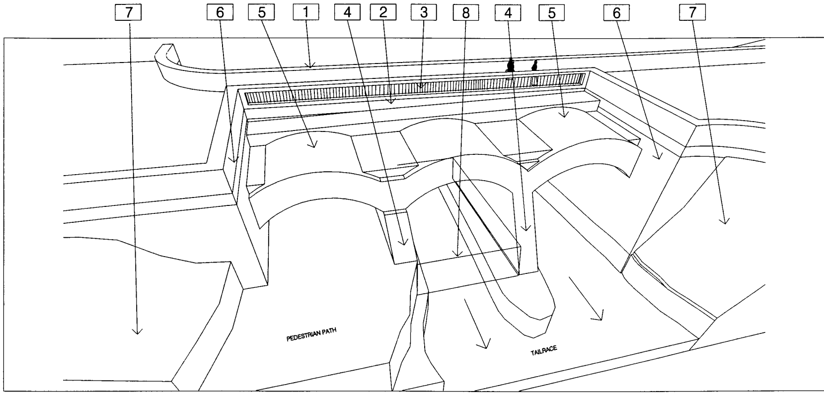
PERSPECTIVE VIEW FROM NORTH
